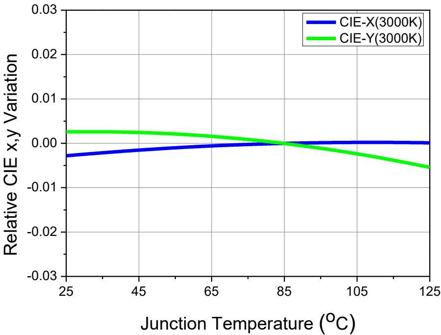
Fig 8. Junction Temperature vs. CIE x,y Shift, I_F=1.05A (3000K)
