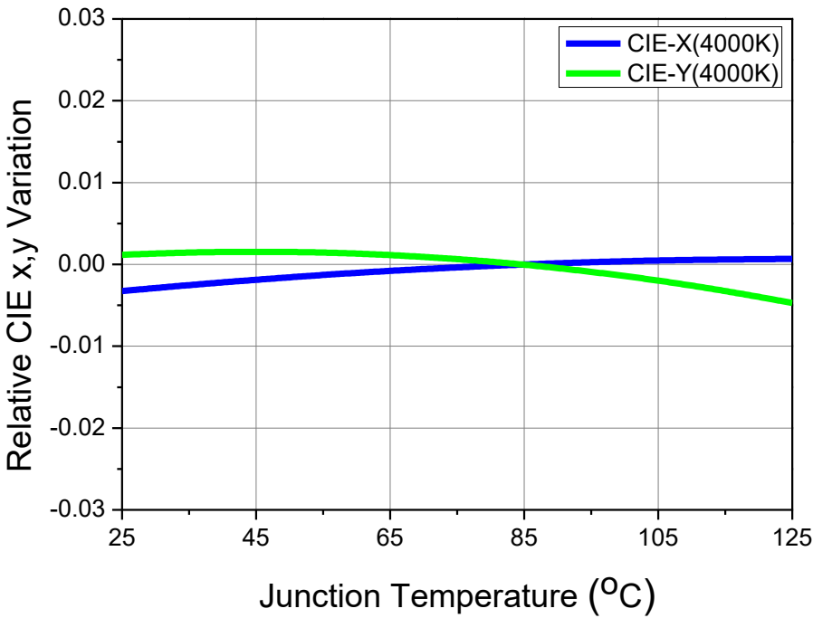
Fig 7. Junction Temperature vs. CIE x,y Shift, I_F=1.05A (4000K)
